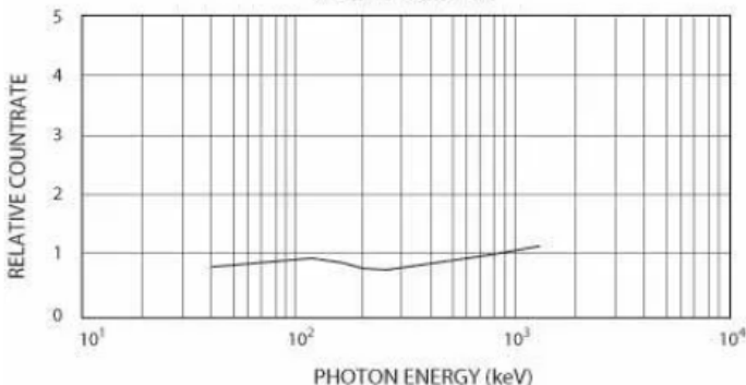
71313 ENERGY RESPONSE (Relative to Cs-137)
